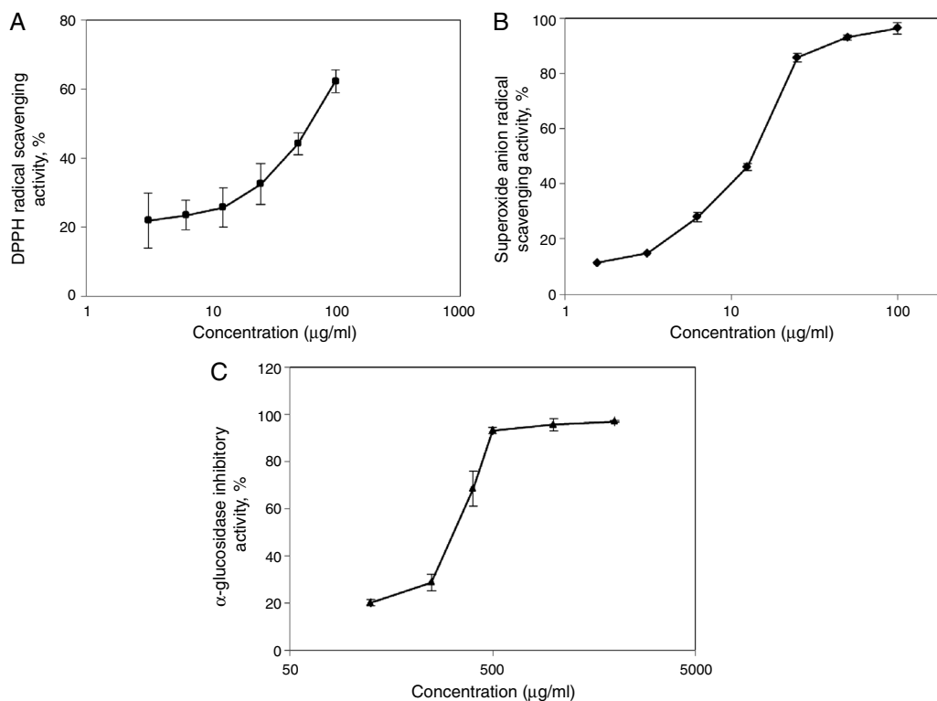
Fig. 1. Concentration-dependent inhibitory effects of compound 1 on: (A) the DPPH radical, (B) the superoxide anion ( \text{O}_2^- ), and (C) the \alpha -glucosidase enzyme. The data are expressed as the mean \pm SD of triplicate experiments ( n = 3 ), and each experiment consists of three repetitions.
